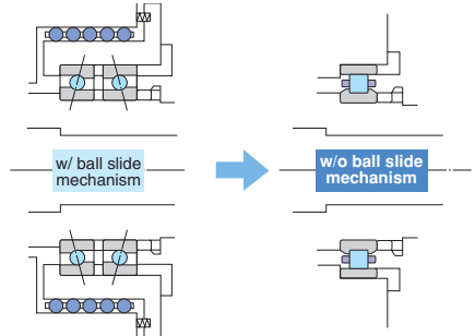
Fig. 10.10 Simplified main spindle rear structure
