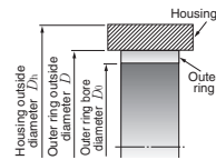
Fig. 6.17 Fit between outer ring and housing
