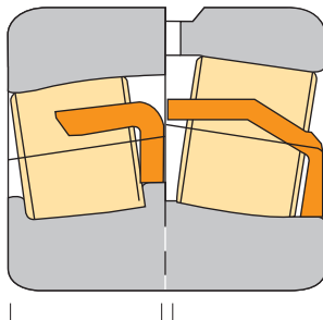
NTN conventional product Type EA
