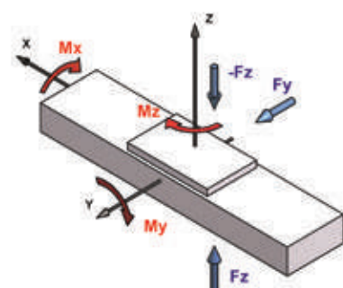
Figure 2.1 ____ Coordinate system
