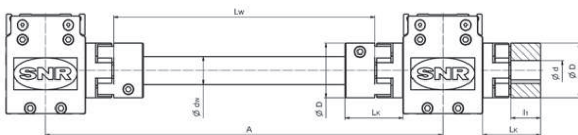
Figure 6.26__ Dimensions couplings and connecting shaft
