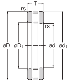
811 812 rulman
