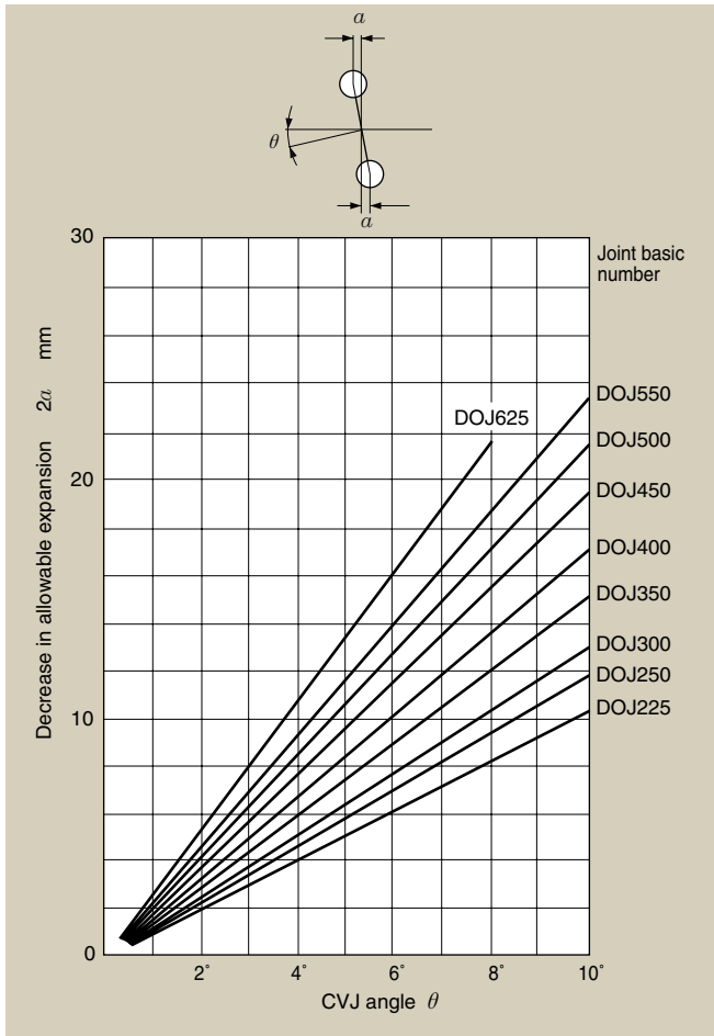
Fig. 16 Allowable expansion
