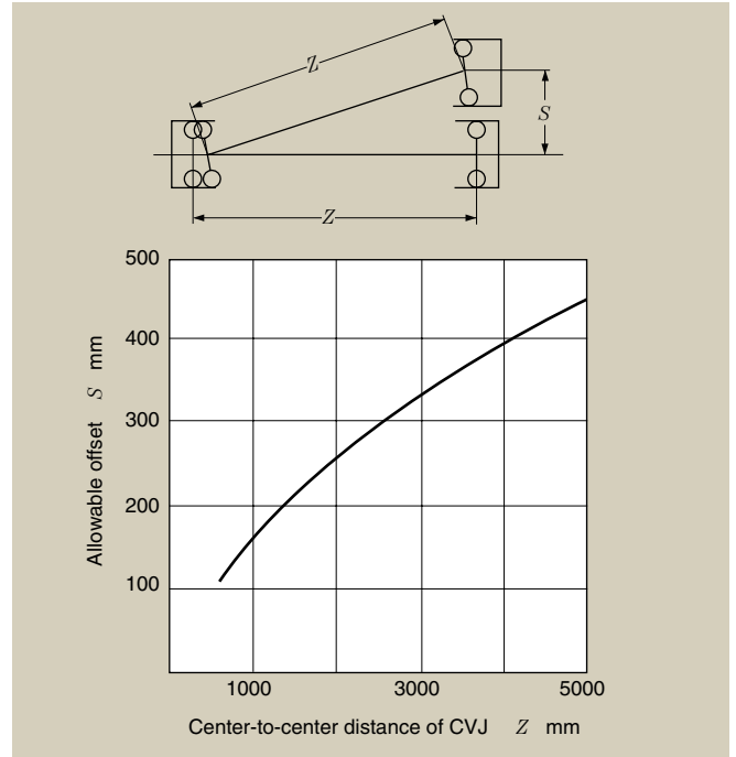
Fig. 17 Allowable offset
