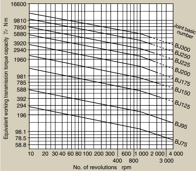
(A) Equivalent working transmission torque capacity
