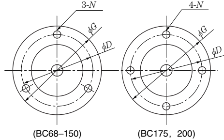
Fig. 5 Coupling (BC68-200) 150 series
