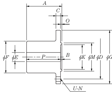
Fig. 4 Cup (BJ75-225) 400, 800 series
