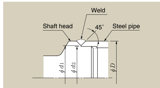
Recommended weld dimensions with steel pipe
